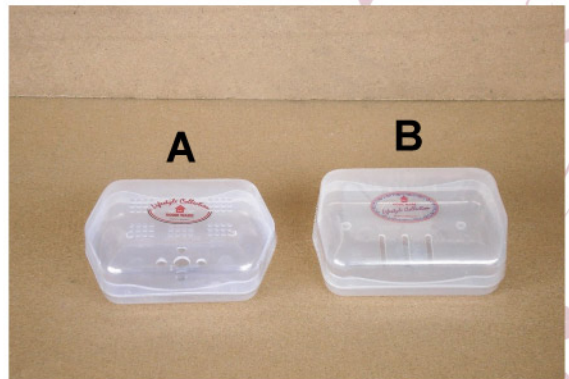
A. 9100/T 115mm X 80mm X 42mm B. 9200/T 118mm X 80mm X 45mm
