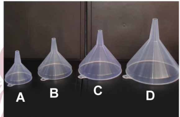
A. 7003/T Ø 76mm (3 inch) X 80mm B. 7004/T Ø 102mm (4 inch) X 100mm C. 7005/T Ø 124mm (5 inch) X 120mm D. 7006/T Ø 153mm (6 inch) X 166mm
