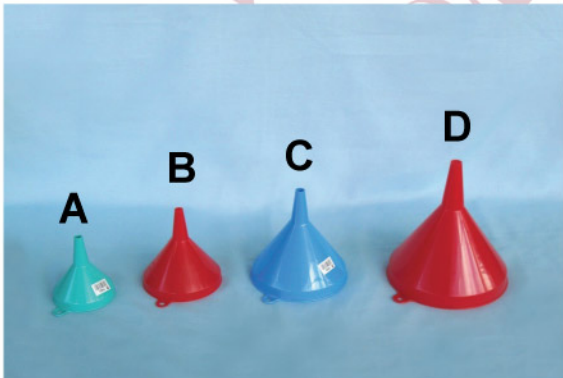
A. 7003 Ø 76mm (3 inch) X 80mm B. 7004 Ø 102mm (4 inch) X 100mm C. 7005 Ø 124mm (5 inch) X 120mm D. 7006 Ø 153mm (6 inch) X 166mm
